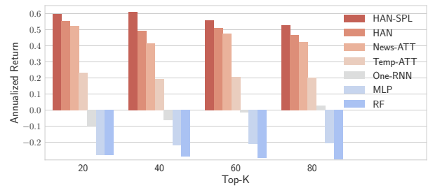
Figure 9: The annualized return for different methods.
